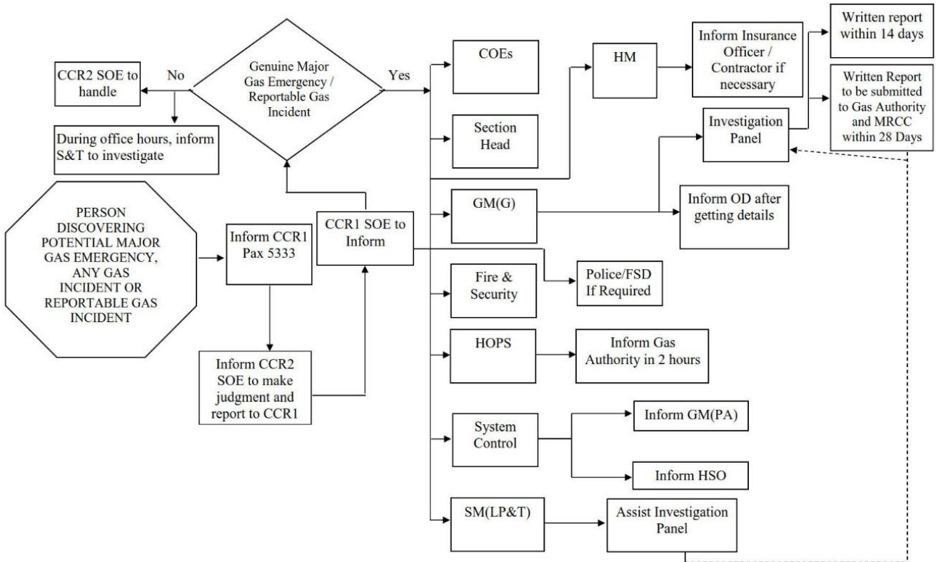
Figure 4.1 Procedure Flowchart – Reporting of an Accidental Event
