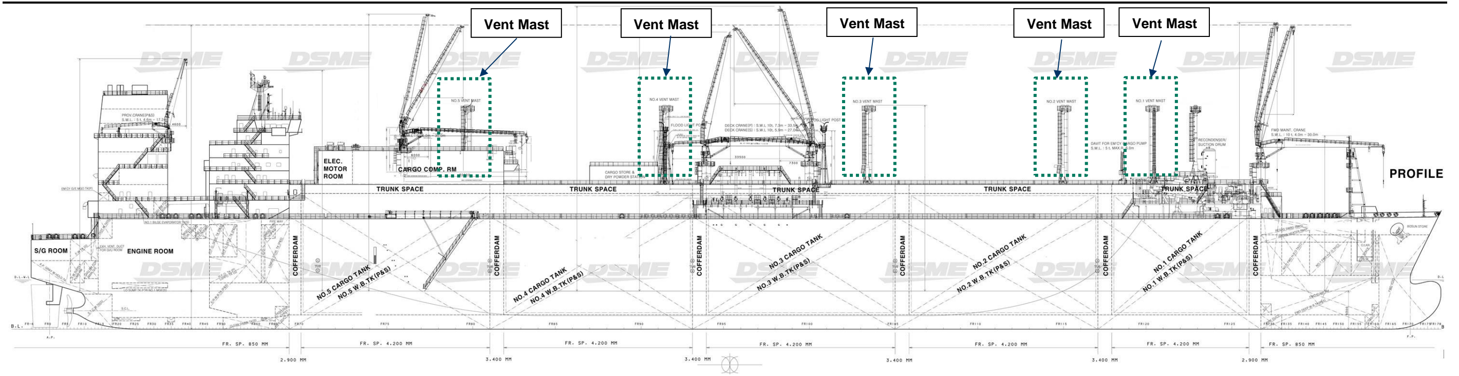
Figure 1.3 Vent Masts of the FSRU Vessel
