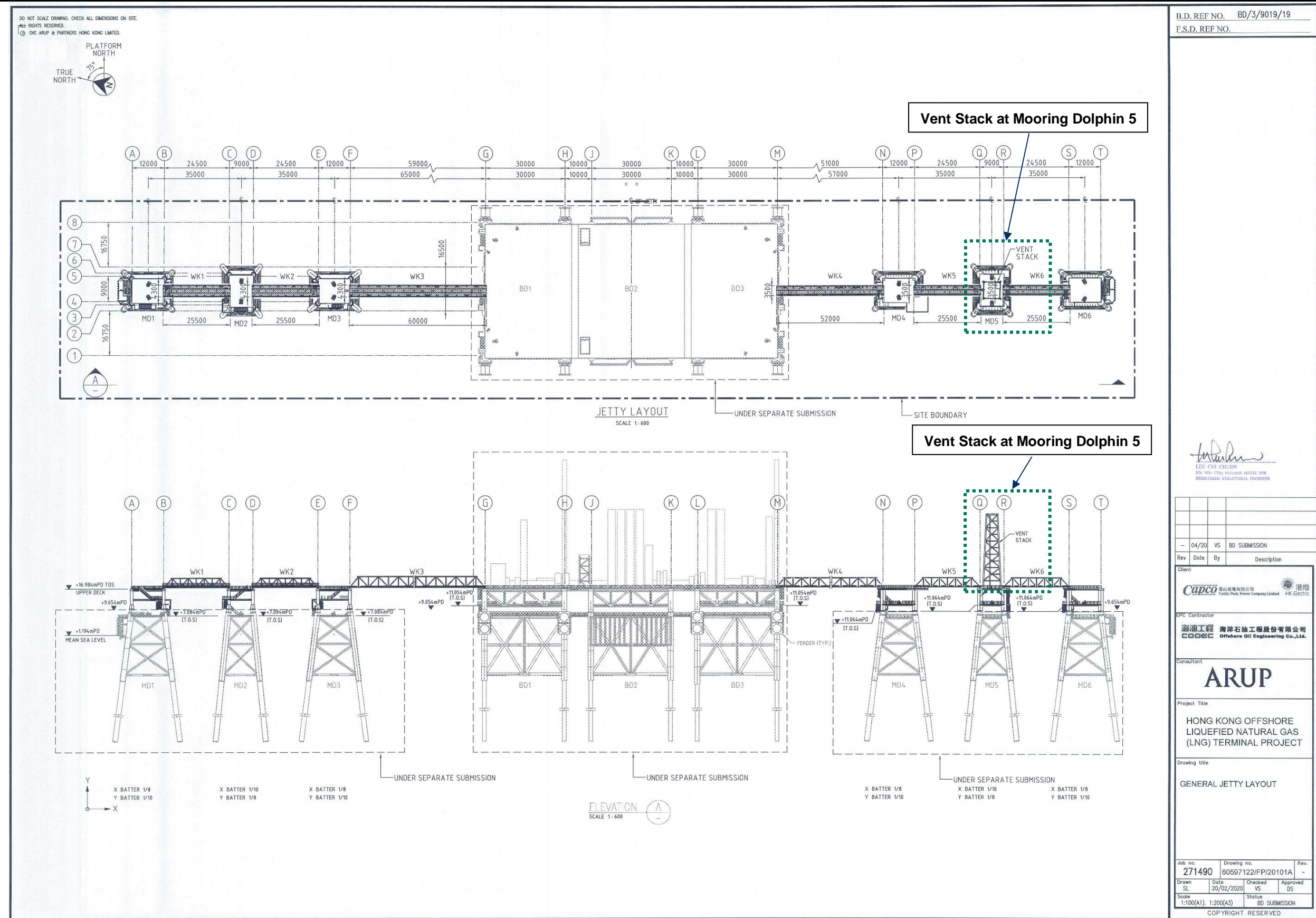
Figure 1.2 The Cold Vent Stack at Mooring Dolphin 5 of the Double Berth Jetty
